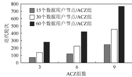
Fig.11 Average number of rounds with varying ACZ groups and number of data users in each ACZ 图 11 ACZ 组数和每个 ACZ 中数据用户节点数量对迭代轮次的影响
