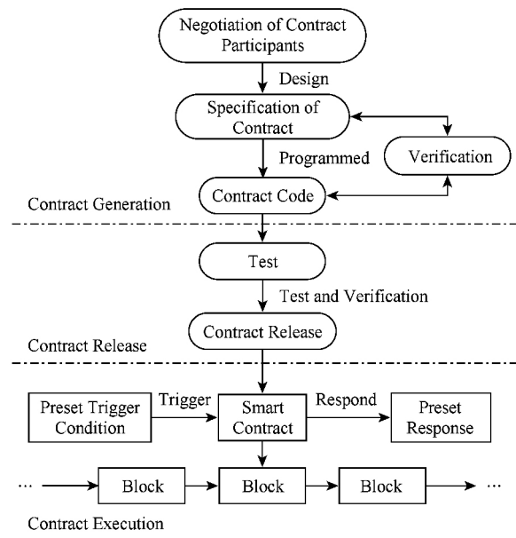
Fig. 2 The whole life cycle of smart contract 图 2 智能合约全生命周期图
